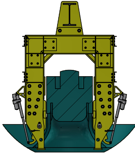
Arms actuated to fit over Spider
