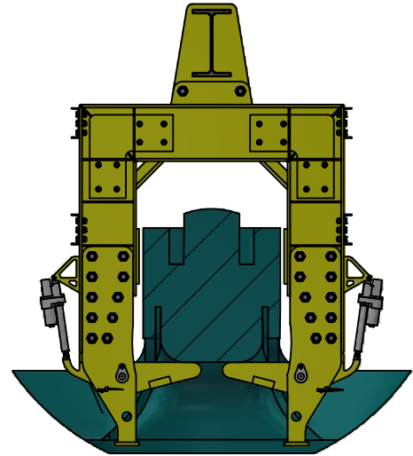
Arms actuators retracted to pick up Spider
