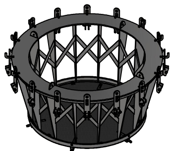
Row 2 Assembly
