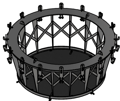
Row 3 Assembly
